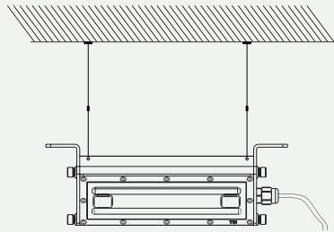
Suspension Installation
