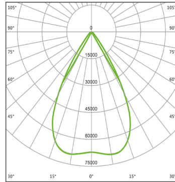
60° PC Lens
