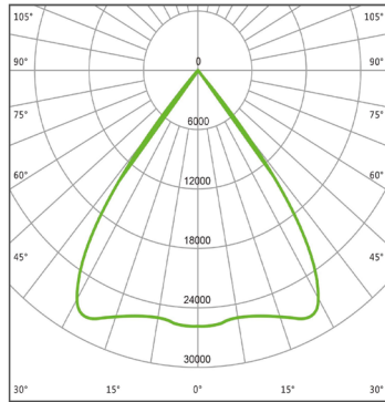
90° PC Lens
